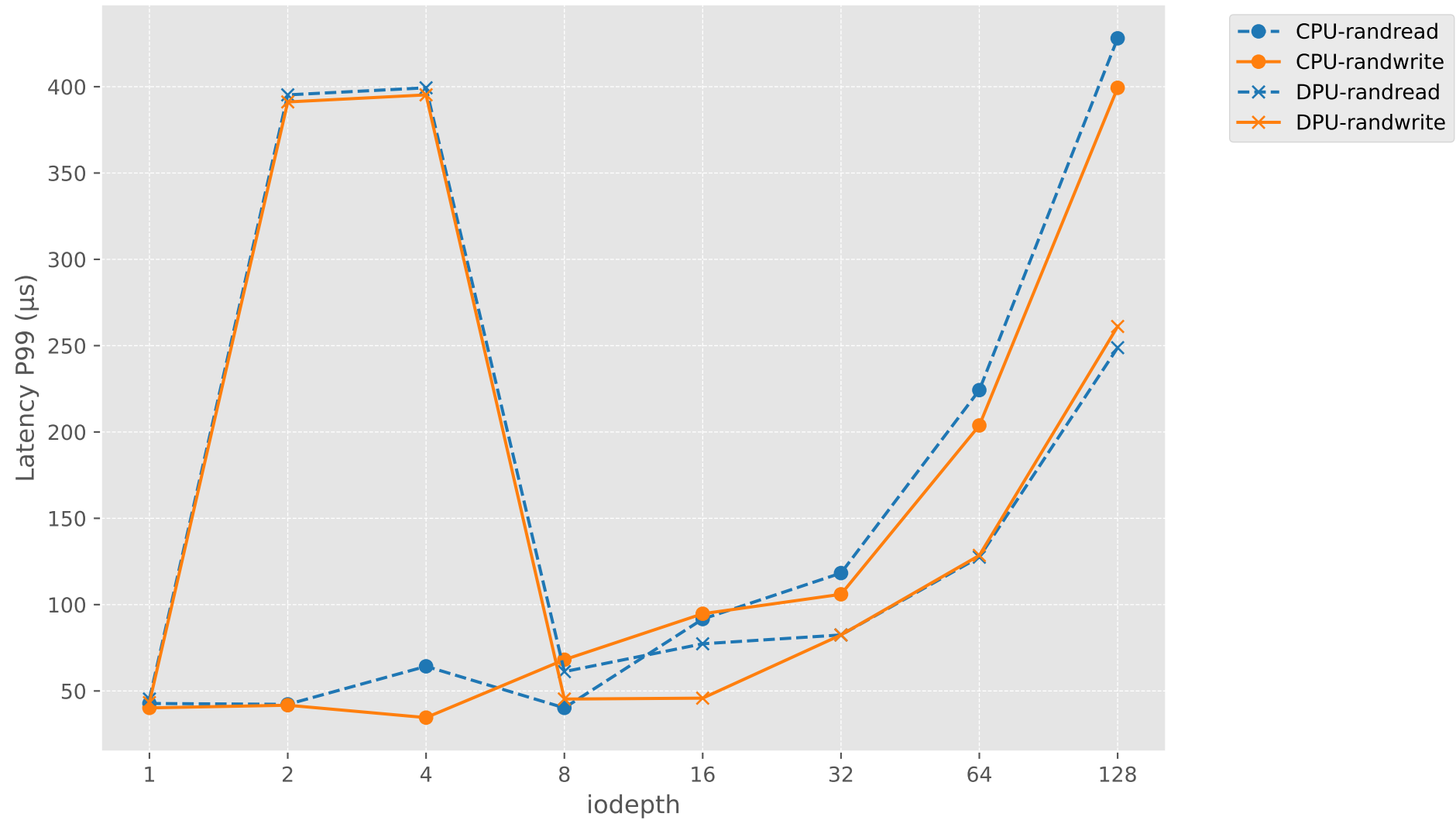
Latency P99 vs iodepth (Random)
